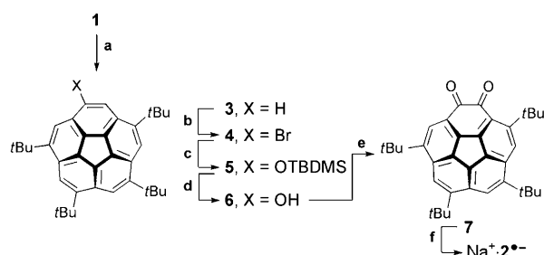
Scheme 1. Synthesis of \text{Na}^+\cdot 2^- : a) t\text{BuCl} , \text{AlCl}_3 , 0^\circ\text{C} , 62 % (estimated by ^1\text{H} NMR spectroscopy); b) \text{Br}_2 , \text{FeBr}_3 , \text{CH}_2\text{Cl}_2 , -78^\circ\text{C} , 98 % (estimated by ^1\text{H} NMR spectroscopy); c) \text{NaOTBDMS} , [\text{Pd}(\text{dba})_2] , ( S )-Tol-BINAP, toluene, 120^\circ\text{C} , 45 % (estimated by ^1\text{H} NMR spectroscopy); d) \text{Bu}_4\text{NF} , THF, room temperature, 100%; e) \text{Ag}_2\text{O} , toluene, 90^\circ\text{C} , 21 %; f) sodium mirror, 2-methyl-THF, room temperature. TBDMS = tert -butyldimethylsilyl, dba = dibenzylideneacetone, ( S )-Tol-BINAP = ( S )-(-)-2,2'-bis(di- p -tolylphosphino)-1,1'-binaphthyl.
